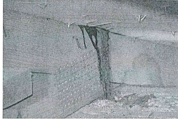
Single strap with 2 nails into the truss
